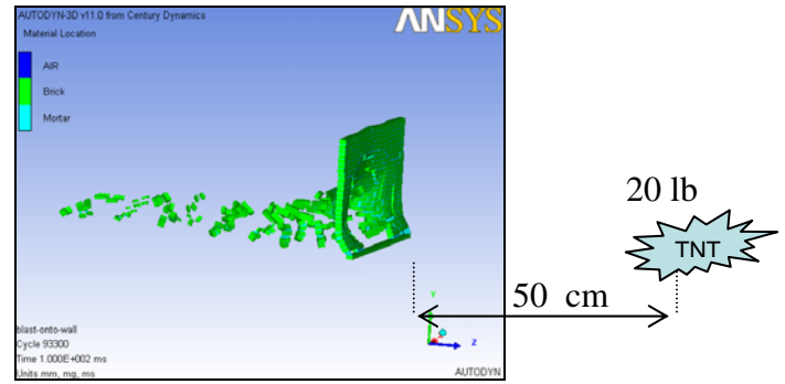
Un-retrofitted brick wall subjected to blast loading
