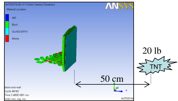
Retrofitted brick wall with FRP subjected to blast loading from the direction of the retrofit
