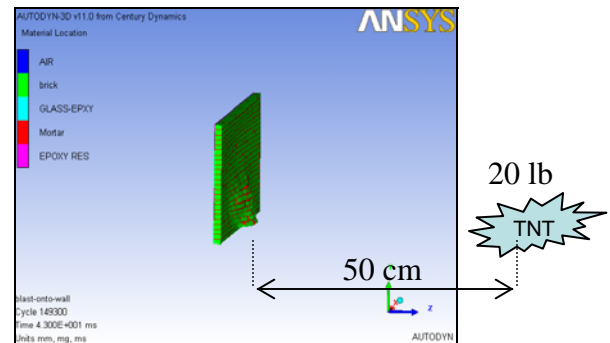
Retrofitted brick wall with FRP subjected to blast loading from the opposite direction of the retrofit
