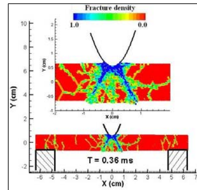
Impact on a 2D polymeric material body
