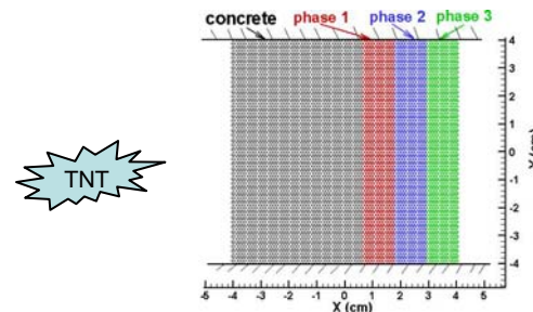
Blast of retrofitted concrete wall
