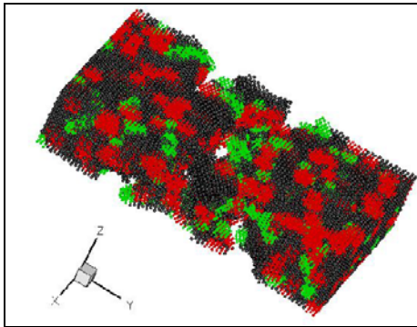
A 3D heterogeneous material body in tension
