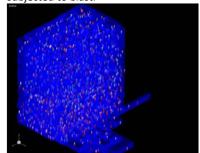
Agent-based evacuation simulation for a nano-particle-reinforcement retrofitted building.
