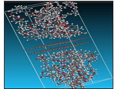
xGNP (exfoliated graphene nano particle) embedded in vinyl ester
