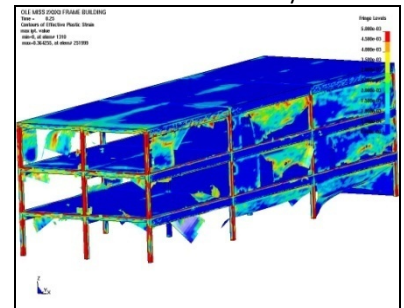
LSDYNA simulation showing a building without nano-particle-reinforcement subjected to blast.
