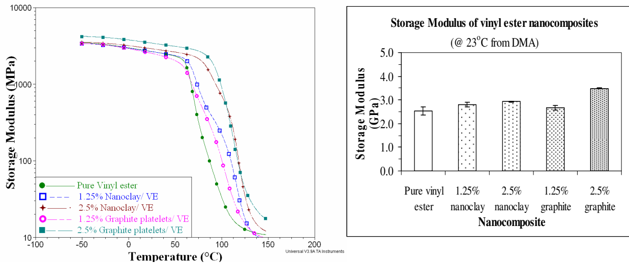
Figure 10: Storage modulus of vinyl ester nanocomposites versus temperature and nano-reinforcement at 23 C from DMA
