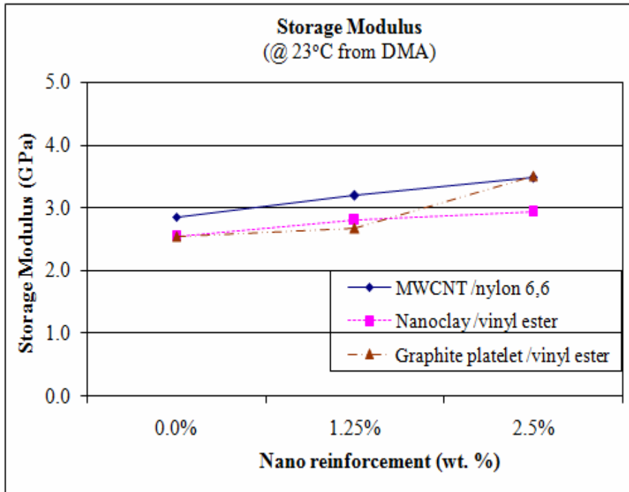
Figure 13: Storage modulus of nylon 6,6 and vinyl ester nanocomposites
