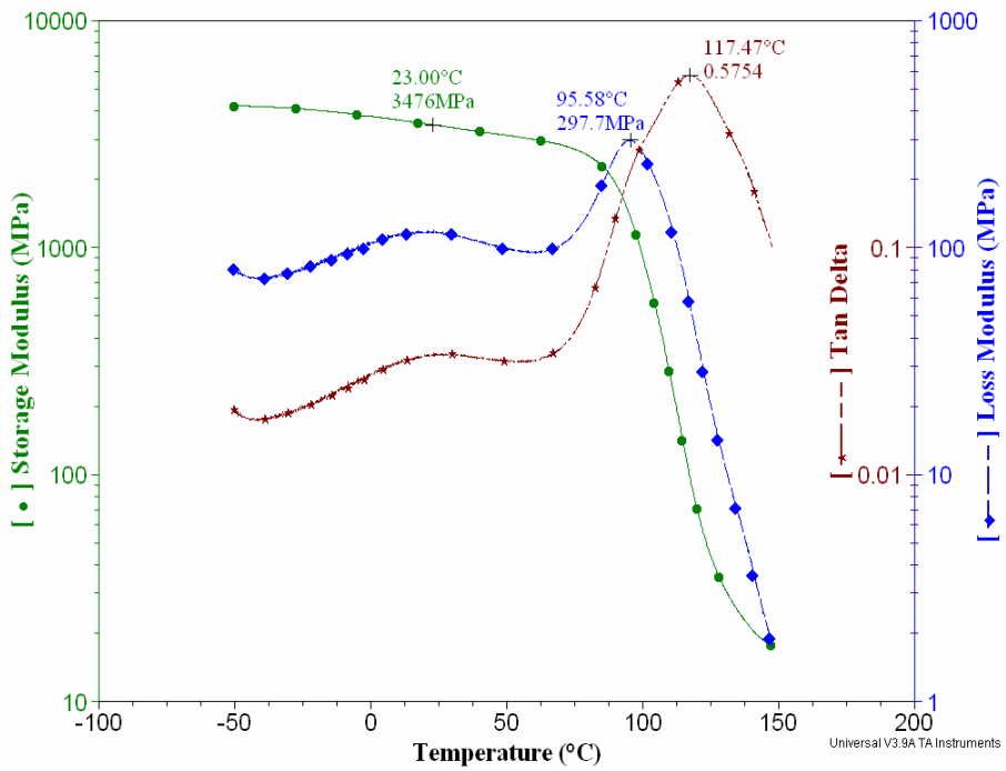
Figure 9: Dynamic modulus and damping for vinyl ester with 2.5 wt. percent graphite platelets
