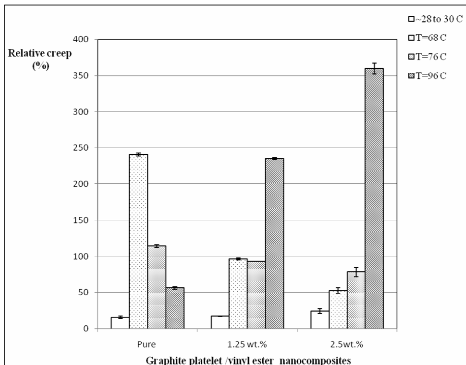
Figure 22: Relative creep for graphite platelet /vinyl ester nanocomposites at various temperatures
