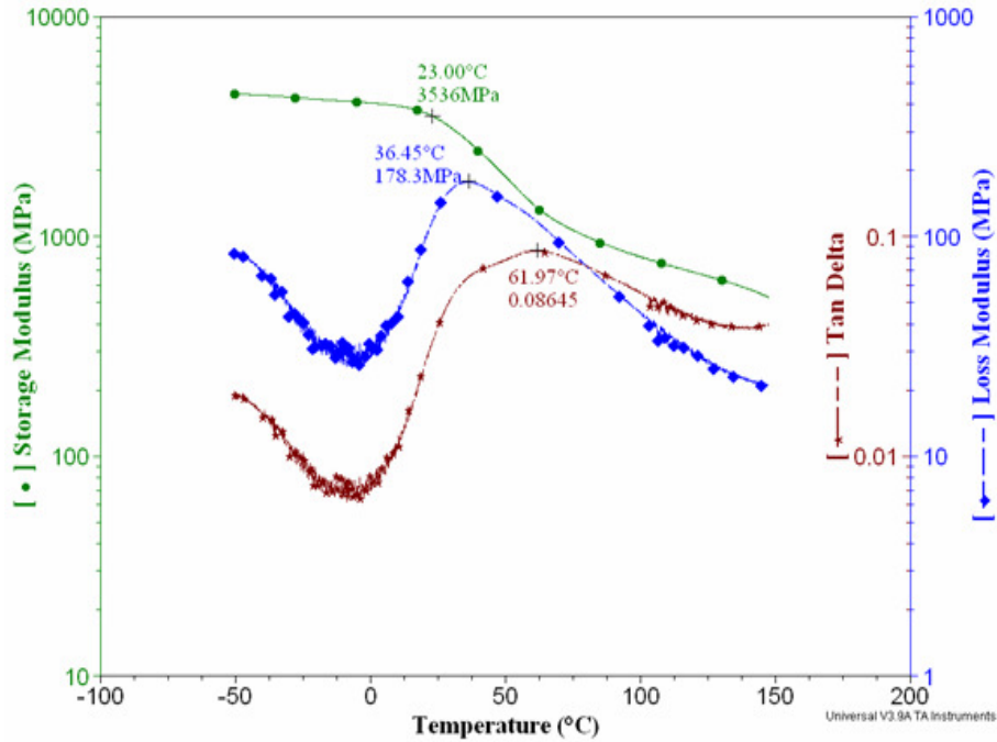
Figure 4: Dynamic modulus and damping of nylon 6,6 with 2.5 wt. percent MWCNT
