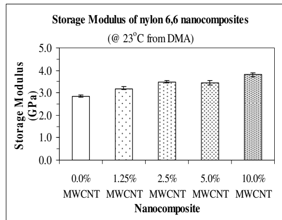
Figure 5b: Storage modulus of MWCNT/nylon 6,6 nanocomposites at 23°C from DMA
