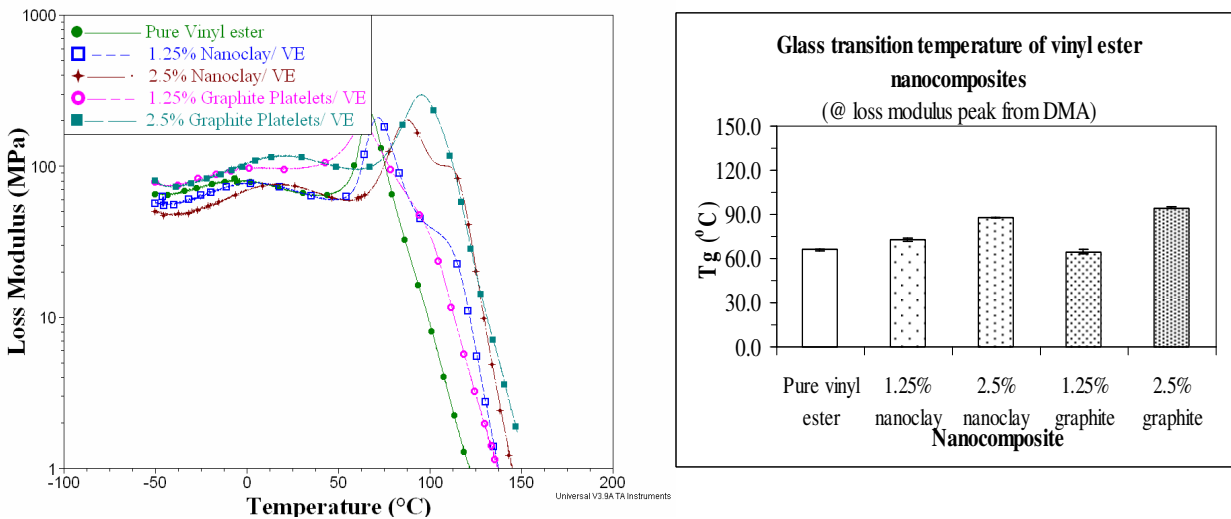
Figure 11: Glass transition temperature of vinyl ester nanocomposites at loss modulus peak from DMA
