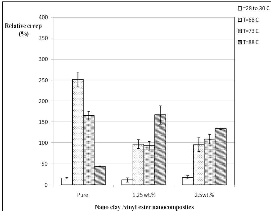
Figure 21: Relative creep for nano clay /vinyl ester nanocomposites at various temperatures
