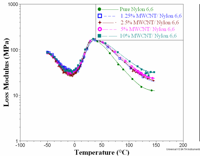
Figure 6a: Loss modulus of MWCNT/nylon 6,6 nanocomposites vs. temperature from DMA
