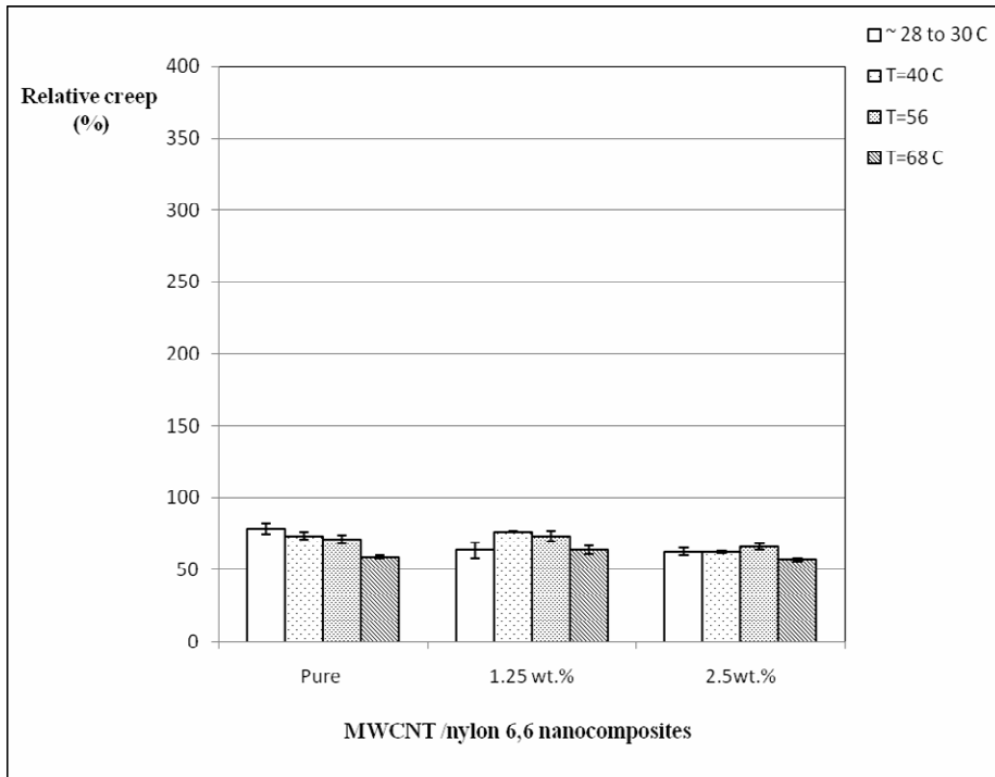
Figure 20: Relative creep for MWCNT /nylon6,6 nanocomposites at various temperatures
