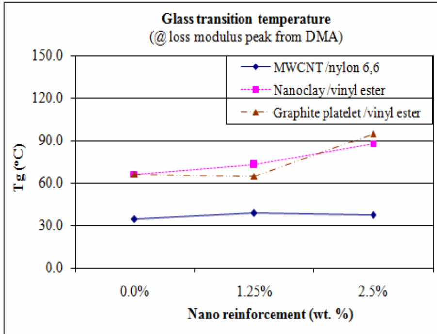
Figure 14: Glass transition temperature of nylon 6,6 and vinyl ester nano composites
