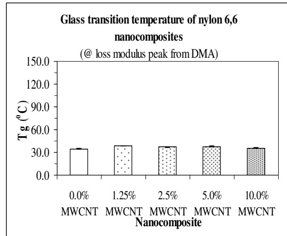
Figure 6b: Glass transition temperature of MWCNT/nylon 6,6 nanocomposites at peak of loss modulus from DMA
