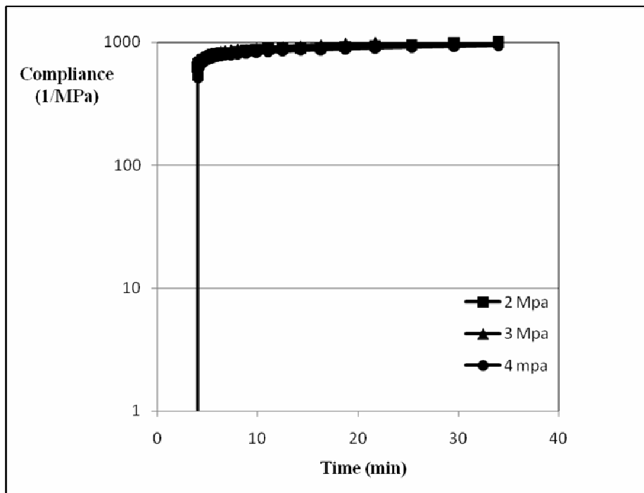
Figure 16: Creep compliance for pure nylon under different (2-4 MPa) preloads
