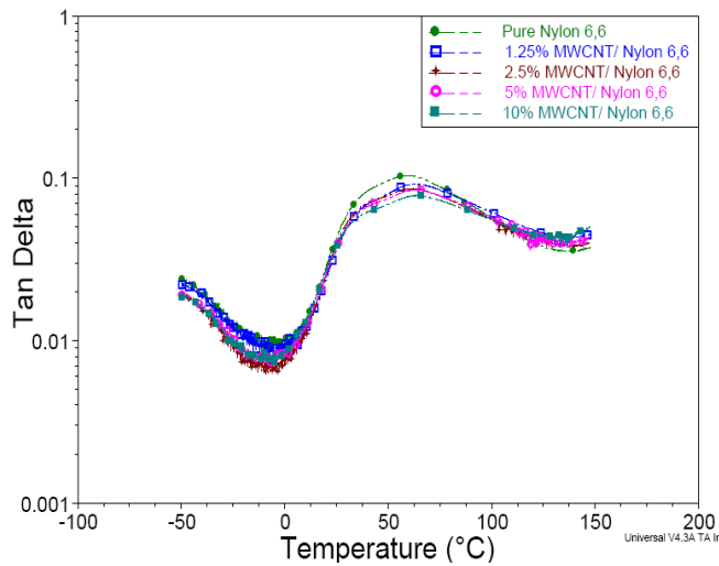
Figure 7a: Tan delta of MWCNT/nylon 6,6 nanocomposites vs. temperature
