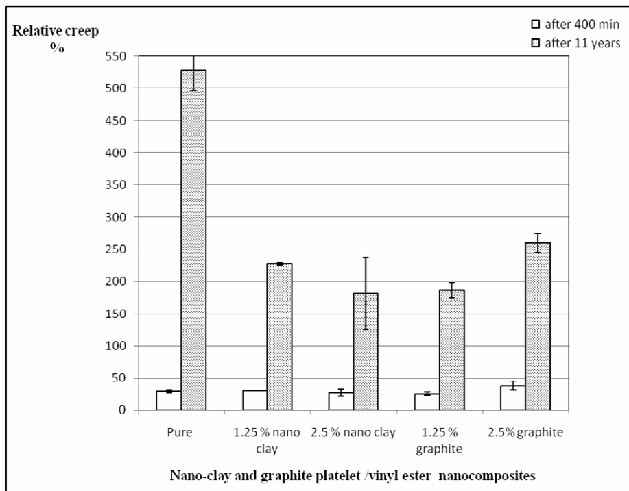
Figure 25: Relative creep for vinyl ester nano clay and graphite nanocomposites generated from shifting of creep data at different temperatures to reference temperature (~ 28 to 30C)
