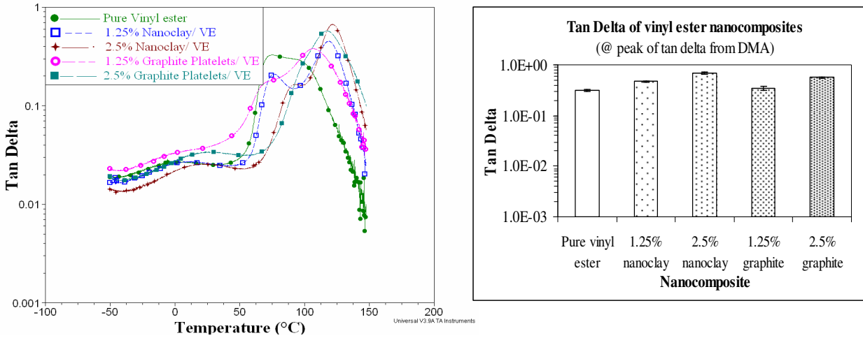
Figure 12: Loss factor of vinyl ester nanocomposites at peak of \tan \delta from DMA
