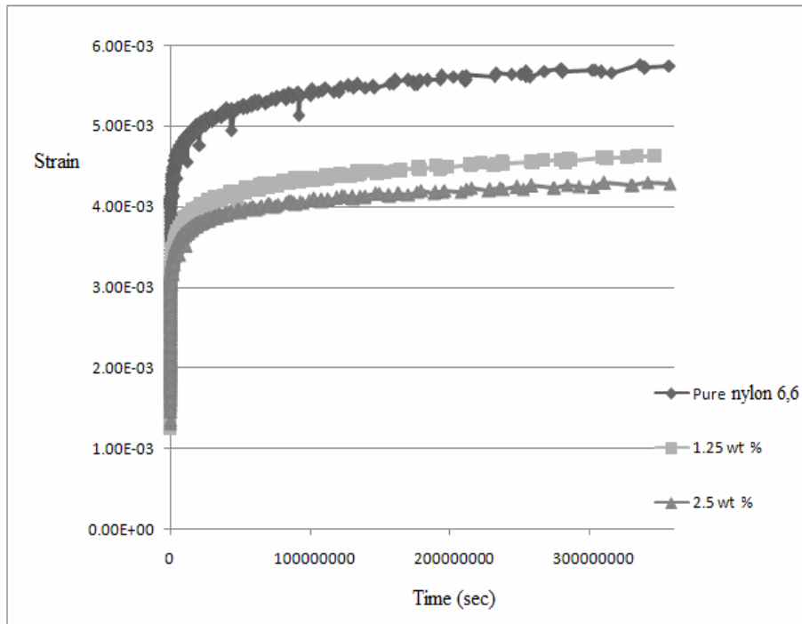
Figure 23: Master curve of creep strain generated by shifting of creep data at different temperatures to reference temperature (~ 28 to 30 C) for MWCNT /nylon 6,6 nanocomposites
