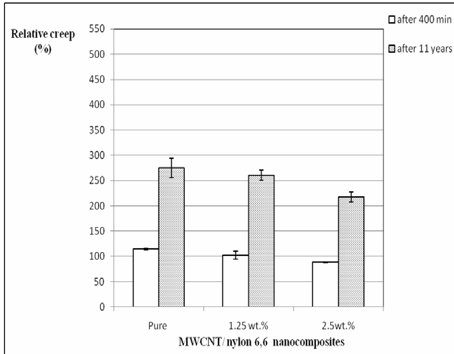
Figure 24: Relative creep for MWCNT /nylon6,6 nanocomposites generated from shifting of creep data at different temperatures to reference temperature (~ 28 to 30 C)
