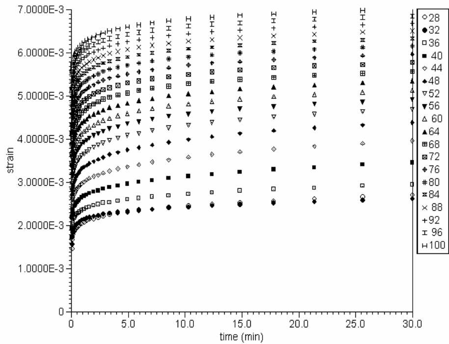
Figure 18: Typical DMA plot of creep-strain for pure nylon 6,6 over 30 min at various temperatures
