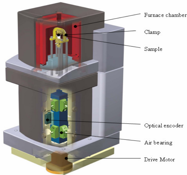
Figure 1: Schematic of TA instruments model Q800 DMA [14]
