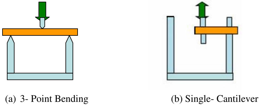
Figure 2: DMA clamps used for testing
