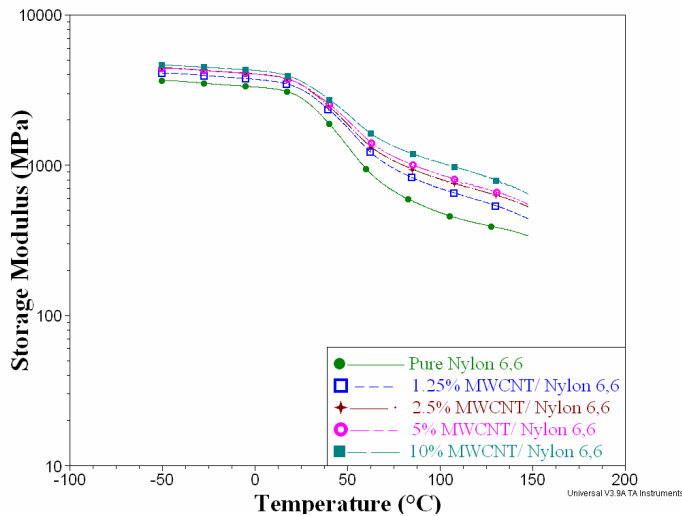
Figure 5a: Storage modulus of MWCNT/nylon 6,6 nanocomposites vs. temperature
