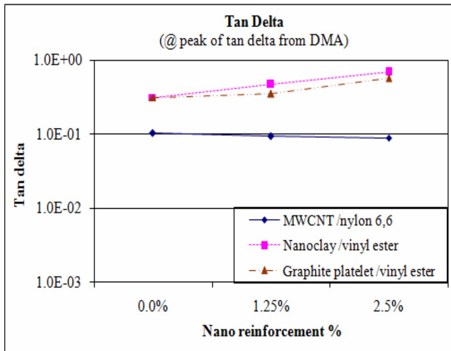
Figure 15: Loss factor of nylon 6,6 and vinyl ester nanocomposites
