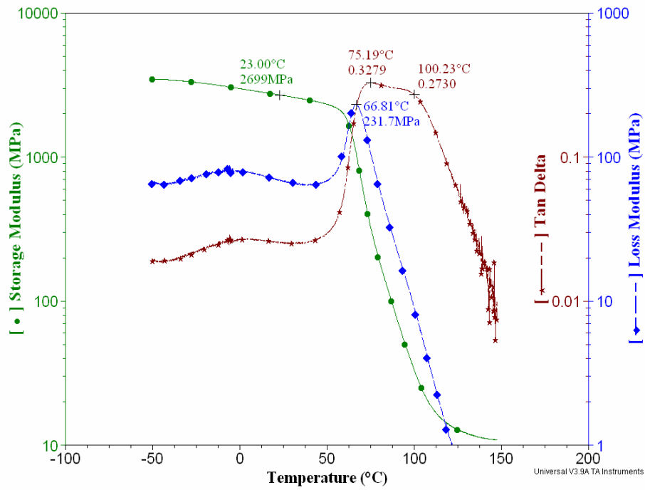
Figure 8: Dynamic modulus and damping for pure vinyl ester
