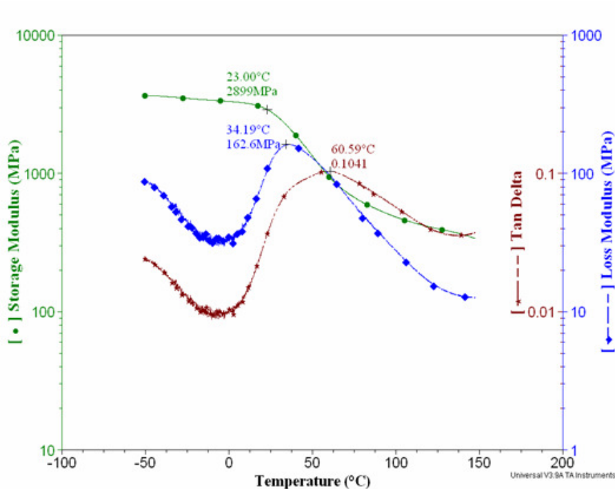
Figure 3: Dynamic modulus and damping for pure nylon 6,6
