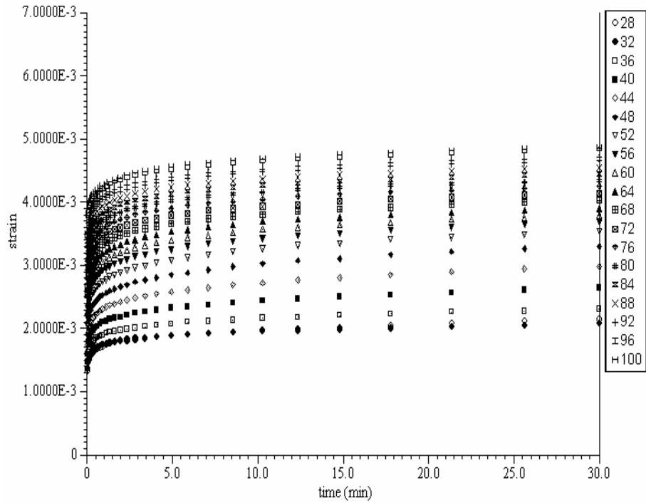
Figure 19: Typical DMA plot of creep-strain for 2.5 wt.percent MWCNT /nylon 6,6 over 30 min at various temperatures
