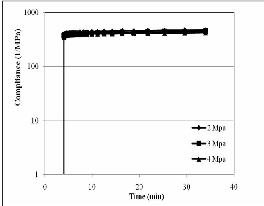
Figure 17: Creep compliance for vinyl ester under different (2-4 MPa) preloads
