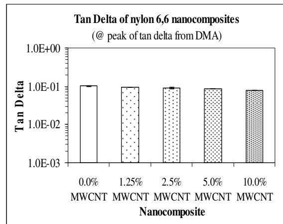
Figure 7b: Loss factor of MWCNT/nylon 6,6 nanocomposites at peak of \tan \delta from
